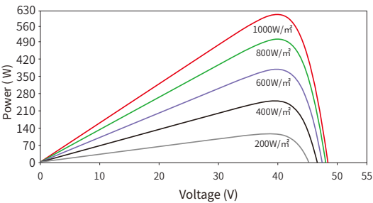
Power-Voltage Curves (615W)
