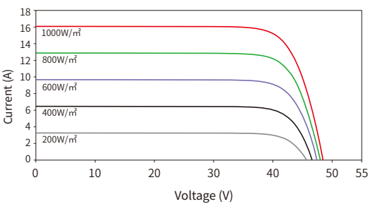
Current-Voltage Curves (615W)
