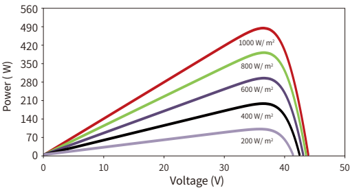
Power-Voltage Curves (490W)
