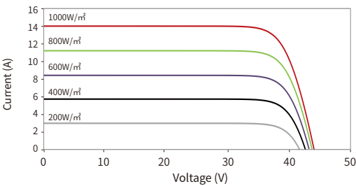
Current-Voltage Curves (490W)
